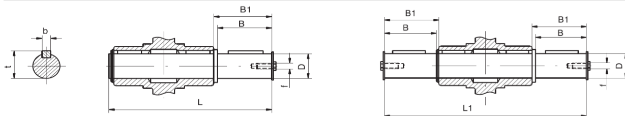
Output shafts
