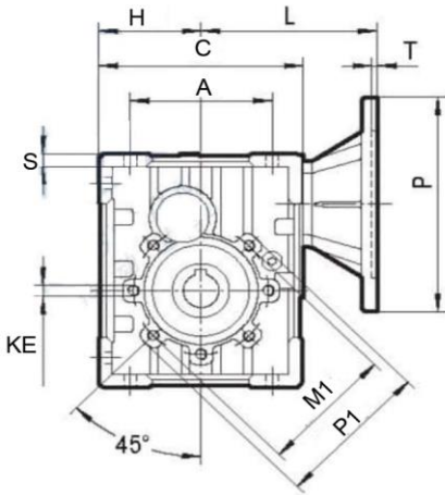
Output Flange
