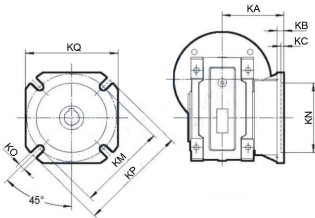
Output Flange
