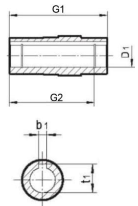
Output Hub
