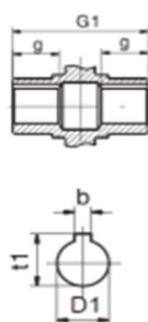
Output Hub
