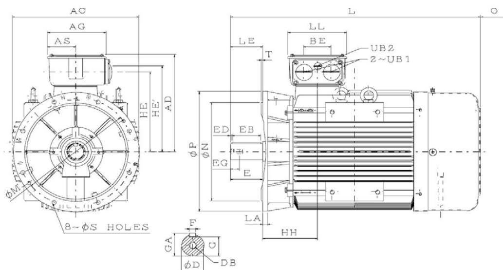
Figure 7-12: Outline drawing of cast iron design, flange version, mounting B5, frame size 160
