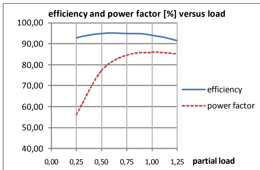
Figure 1-4: Typical characteristic for a TECO motor (30 kW): power factor and efficiency at partial load
