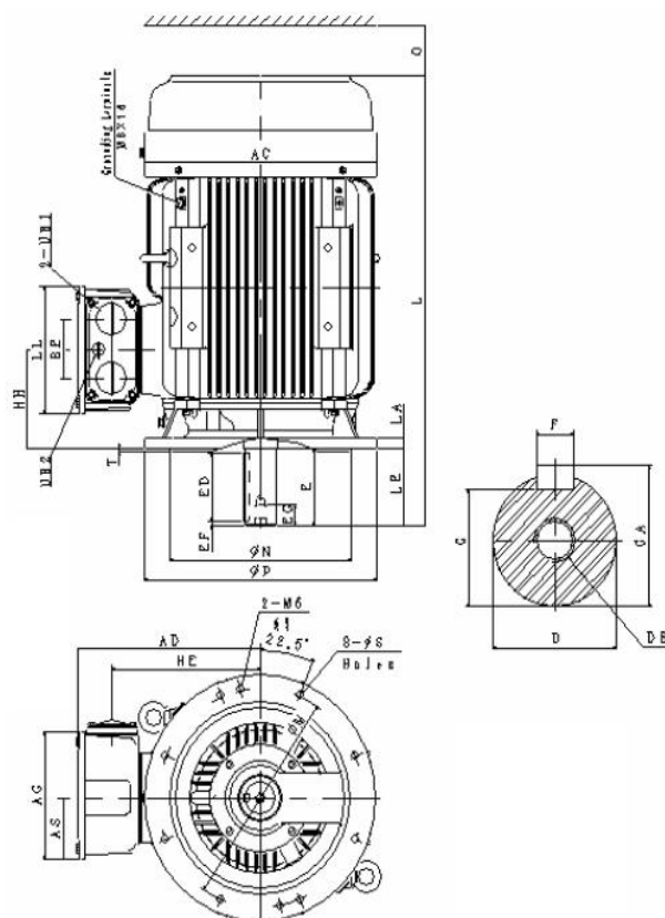
Figure 7-27: Outline drawing of cast iron design, mounting V1; frame size 225 – 250
