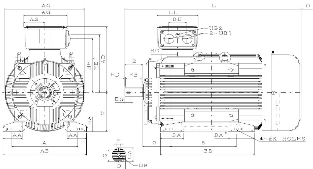
Figure 7-10: Outline drawing of cast iron design, feet version, mounting B3; frame size 315L
