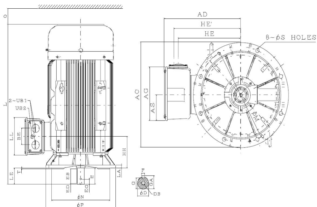
Figure 7-30: Outline drawing of cast iron design, mounting V1; frame size 315L
