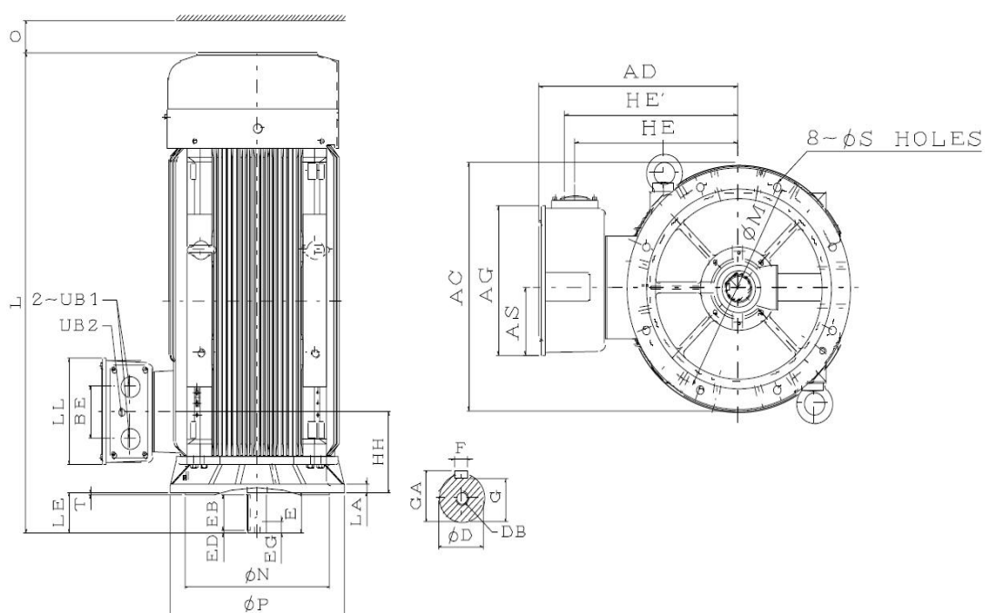
Figure 7-31: Outline drawing of cast iron design, mounting V1; frame size 315D
