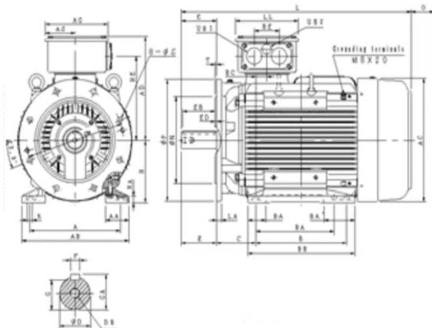
Figure 7-19: Outline drawing of cast iron design, mounting B35; frame size 200 - 250
