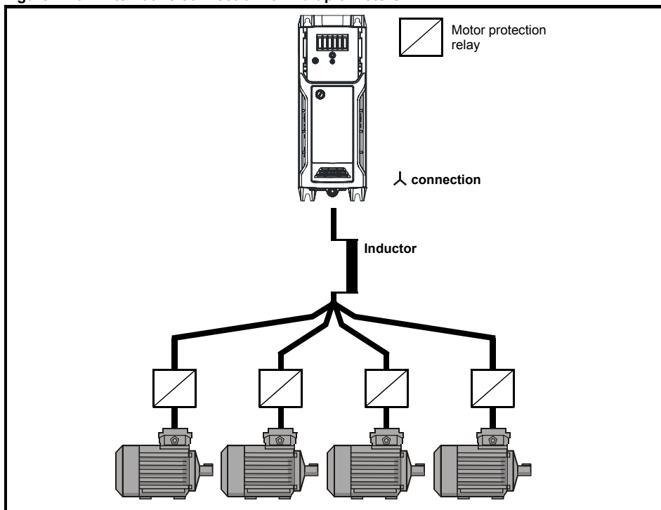
Figure 4-10 Alternative connection for multiple motors
