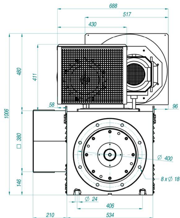
MAC - HS4 250 P Motor Dimensions
