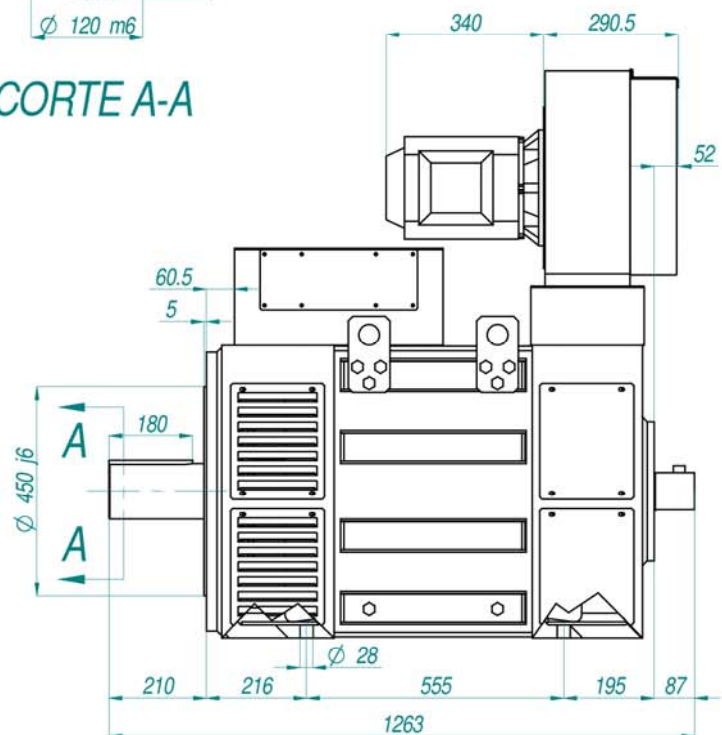
MOTOR MAC QI 315 S DIMENSIONS
