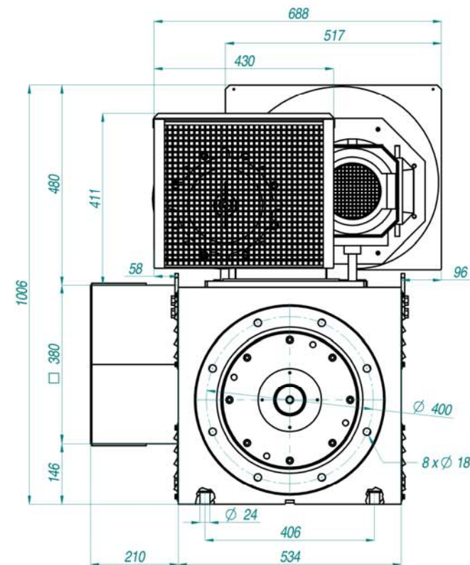
MAC - HS4 250 L Motor Dimensions
