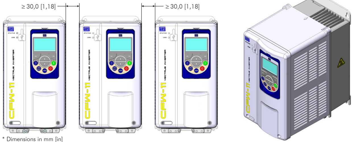
(a) Minimum side clearance requirements
