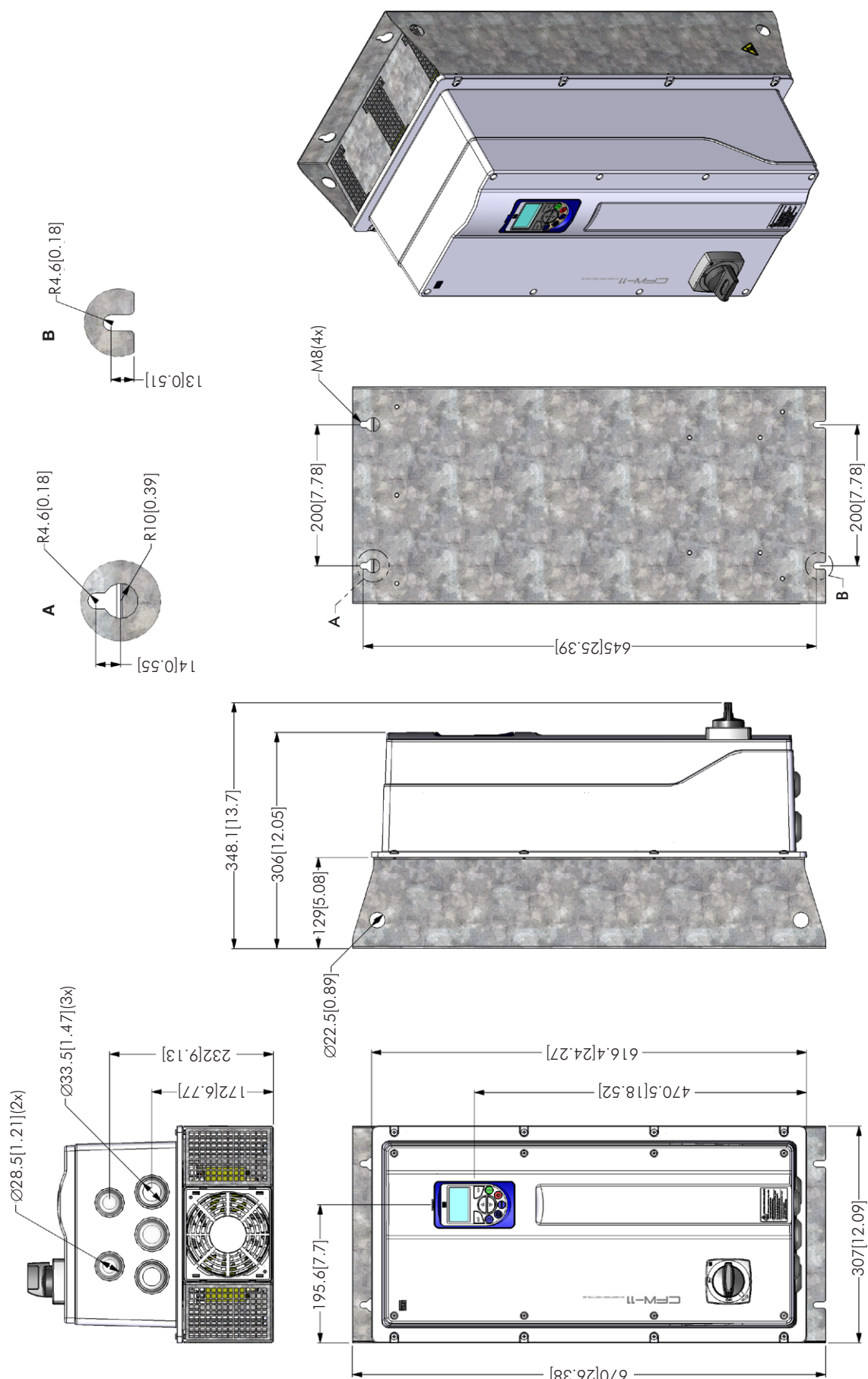
Figure 8.7 - Inverter dimensions - frame size C - mm [in]
