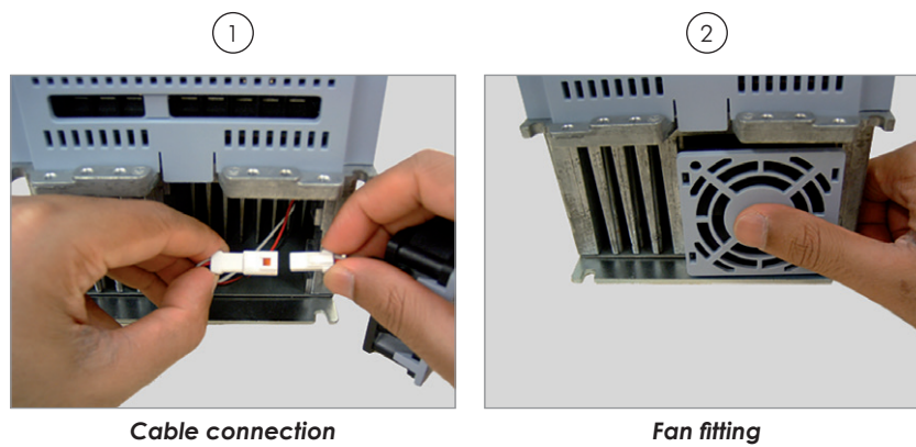
Figure 6.2 - Fan installation
