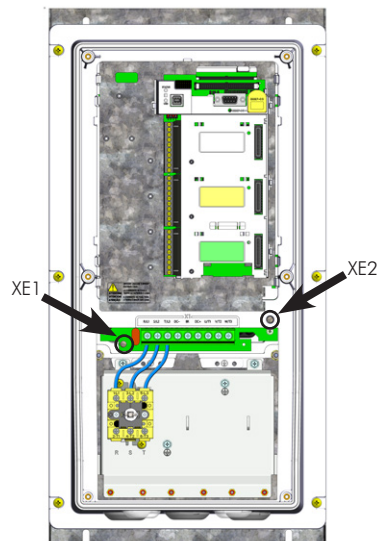
(f) Models 24T2, 28T2, 33T2, 17T4, 24T4 and 31T4 with degree of protection IP55 (frame size B)
