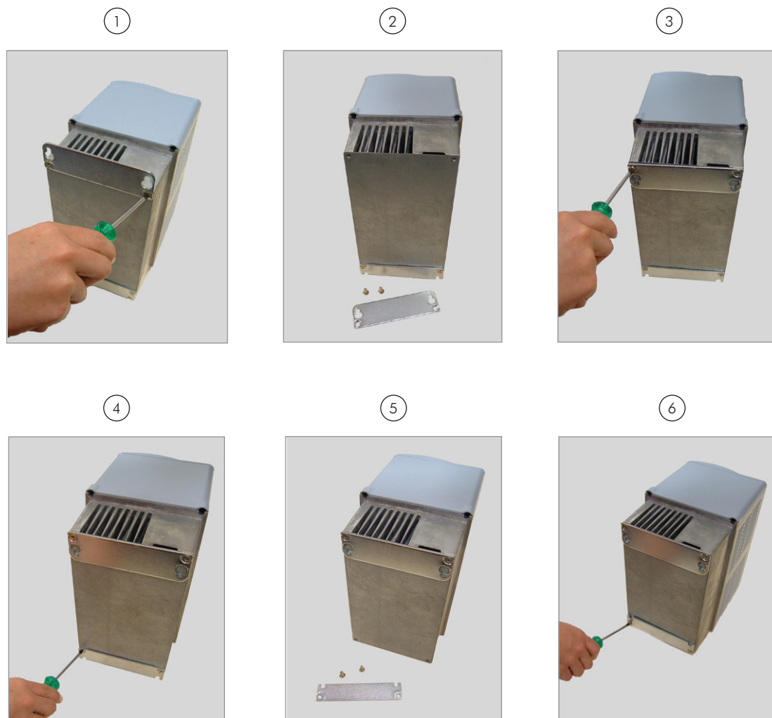
Figure 3.4 - Repositioning the mounting supports
