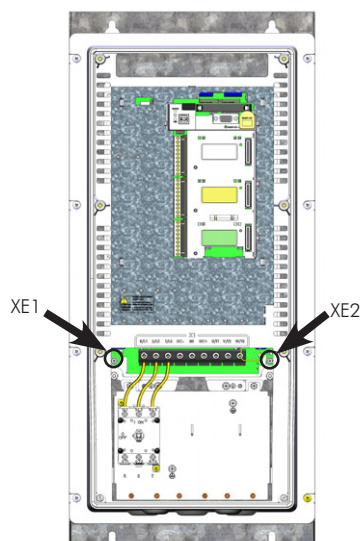
(e) Models up to 16T2 and 13T4 with degree of protection IP55 (frame size B) all of frame size C with degree of protection IP55
