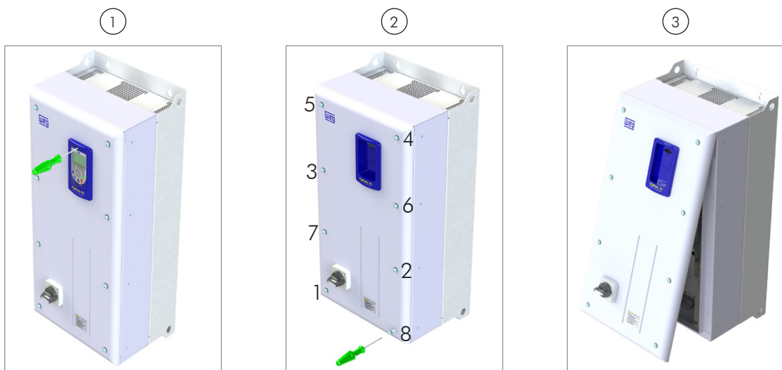
(b.1) Frame sizes B and C
