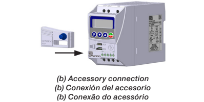
Figure A1: (a) and (b): Installation of accessory Figura A1: (a) y (b): Instalación de accesorio Figura A1: (a) e (b): Instalação de acessório
