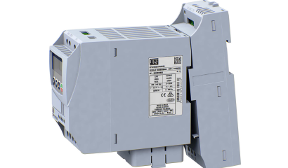
(b) Fit the upper snaps of the filter set into the CFW100 base
