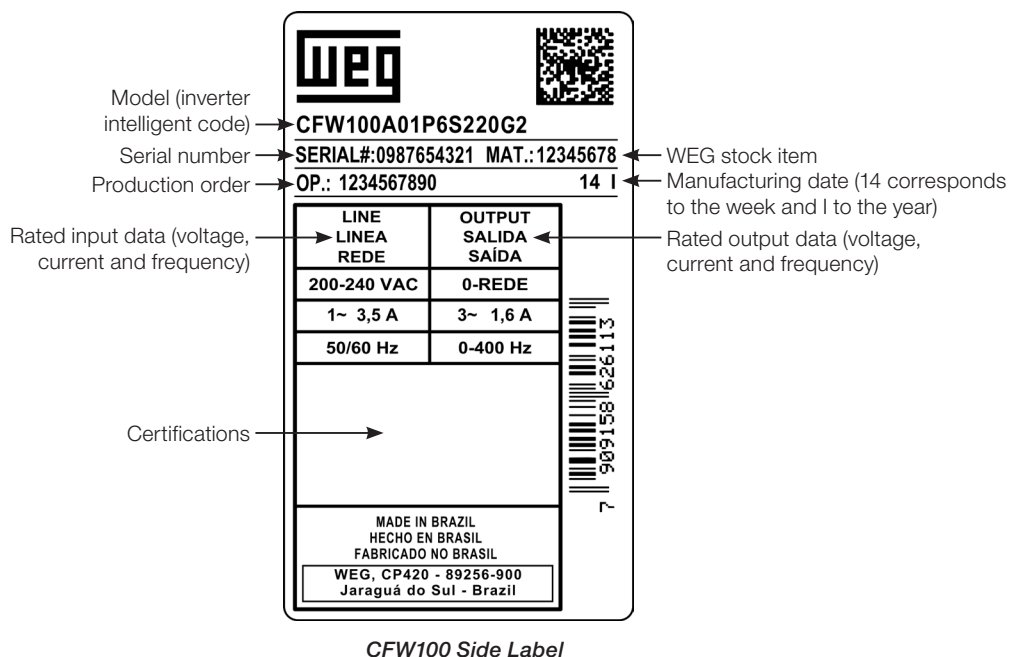
Figure 2.3: Description of the CFW100 identification label
