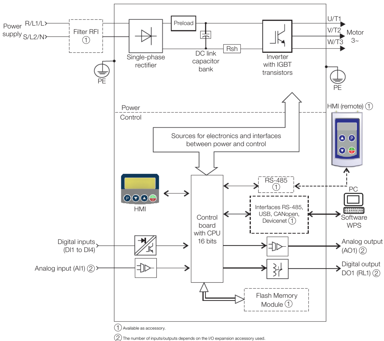
Figure 2.1: CFW100 block diagram for frame size 220 V
