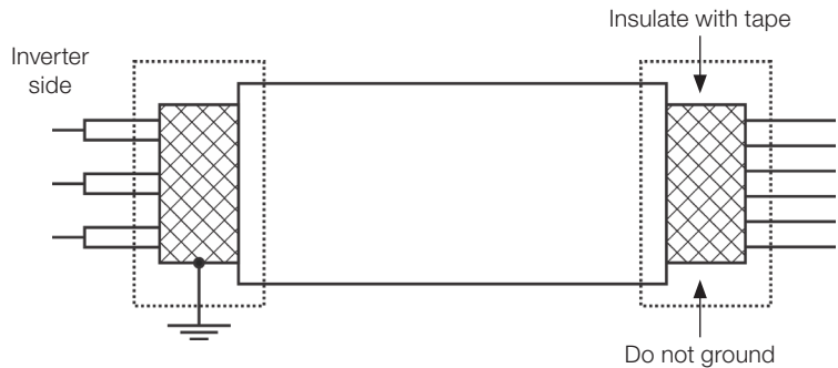
Figure 3.3: Shield connection
