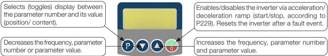
Figure 4.1: HMI keys
