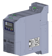
(c) Retract the lower snaps of the filter set into the CFW300 base (c) Retraer as trabas inferiores del conjunto filtro en la base del CFW300 (c) Recolha as travas inferiores do conjunto filtro na base do CFW300
