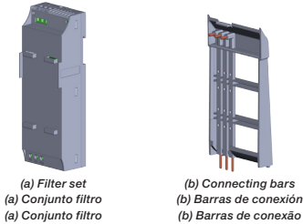
Figure A1: (a) and (b) Parts of the CFW300-KFA filter kit
