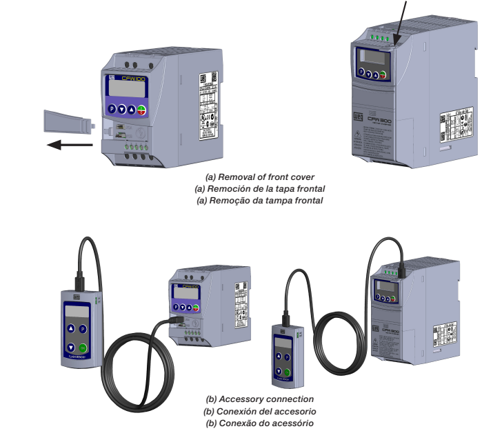
Figure A1: (a) and (b) Installation of accessory Figura A1: (a) y (b) Instalación de accesorio Figura A1: (a) e (b) Instalação de acessório
