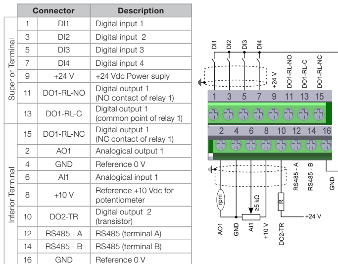
Figure 1: Signals of control connector
