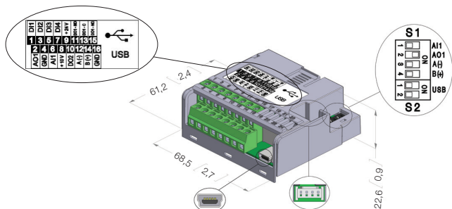
Figure A.2: CFW500-CUSB dimensions in mm [in], DIP-switches location and CFW500-MMF connector Figura A.2: Dimensiones del CFW500-CUSB en mm [in], localización de las DIP-switches y conector de CFW500-MMF Figura A.2: Dimensões do CFW500-CUSB em mm [in], localização das DIP-switches e conector do CFW500-MMF
