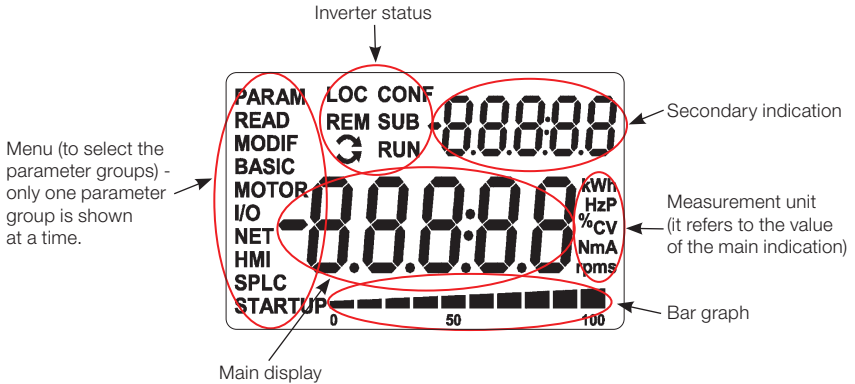
Figure 4.2: Display fields
