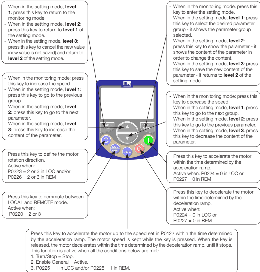
Figure 4.1: HMI Keys
