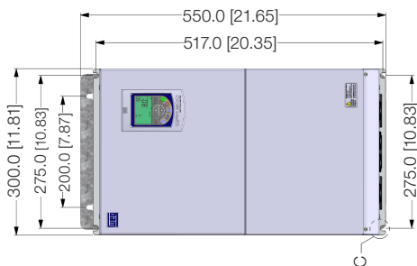
Figure B.10: Inverter dimensions in mm [in] - frame size F
