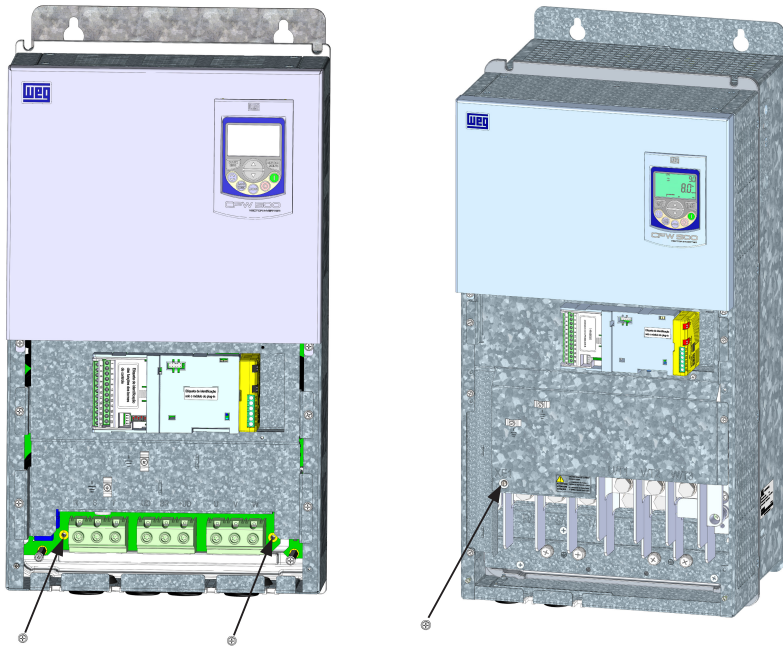
Figure A.4: Location of filter capacitors ground disconnection points - disconnection trough bolts - frame sizes F and G
