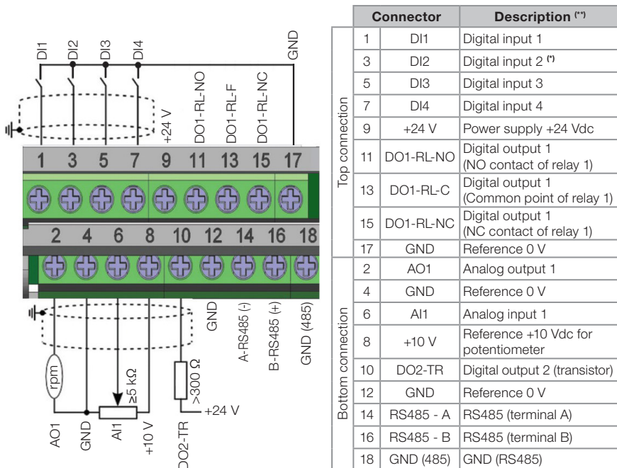
Figure 3.4: Signals of the connector of the CFW500-IOS plug-in module
