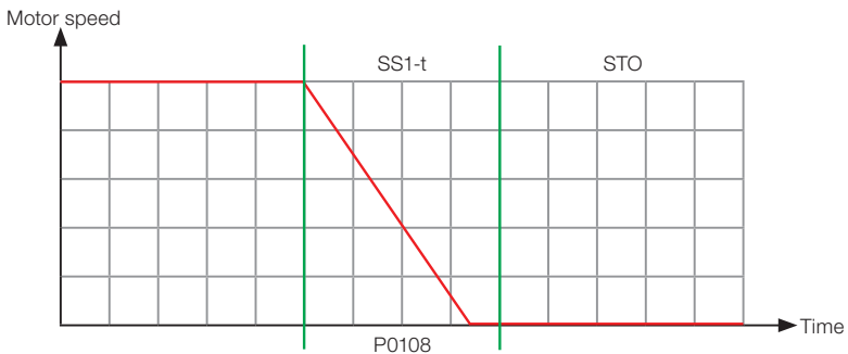
Figure 1.2: SS1-t behavior
