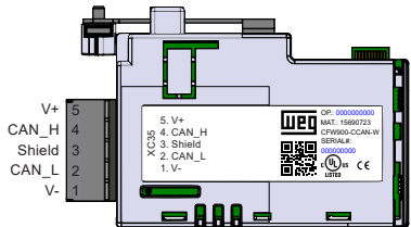
Figure A.2: Pinout of CFW900-CCAN-W
