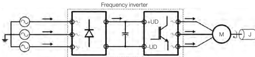
Figure 2.1: Motorization step
