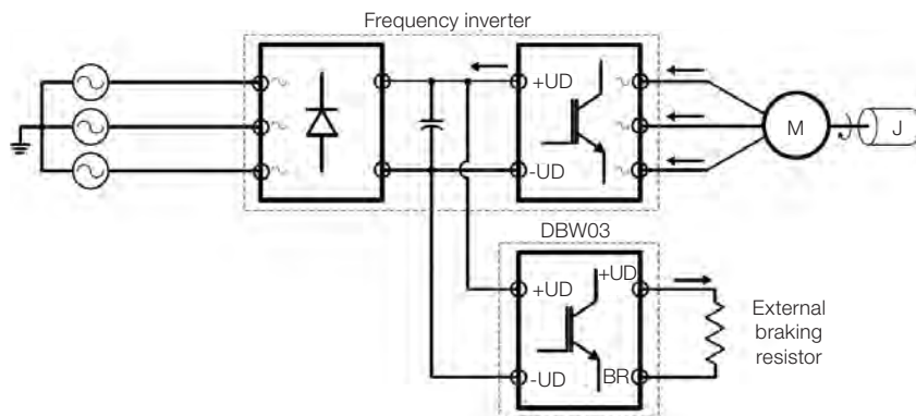
Figure 2.2: Braking step
