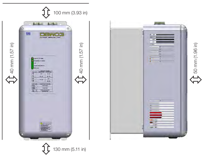
Figure 3.1: Ventilation clearances
