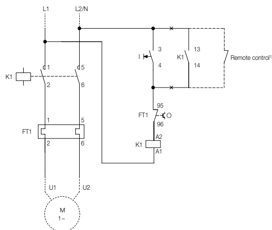
Figure 1 (phase to phase coil supply)
