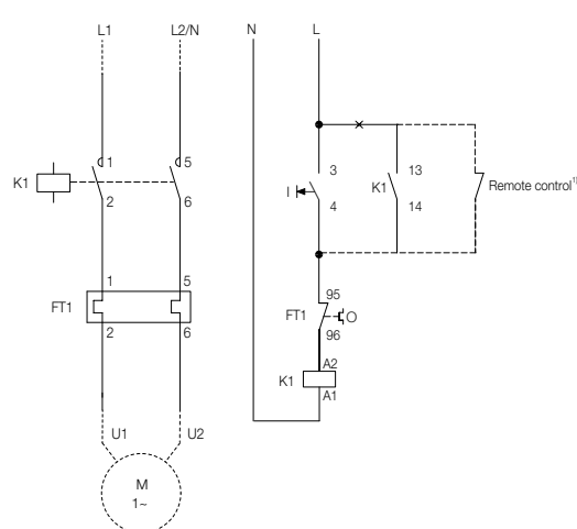
Figure 2 (control circuit connected through a separate coil supply)
