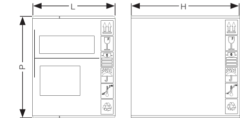
Figure 1: Packing dimensions
