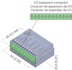
Figure A2: CFW300-IOAR dimensions in mm [in] and connectors location
