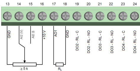
Figure A3: Example of connection of the analog input and output
