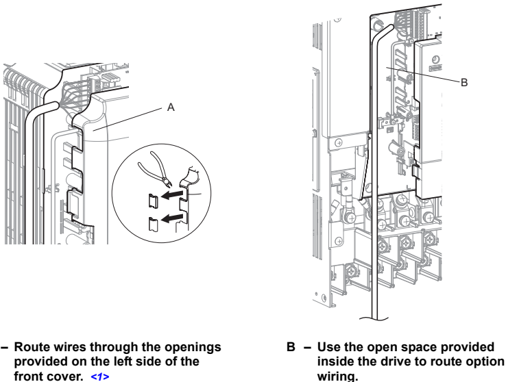
Figure 9 Wire Routing Examples
