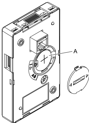
Figure 5.35 Insert the New Battery
