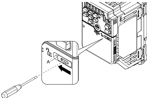
Figure 5.30 Unlocking
