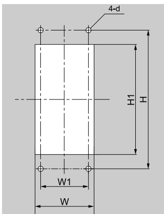
Figure 5.27 Internal/Flush-Mount Enclosure Panel Cut-Out Dimensions
