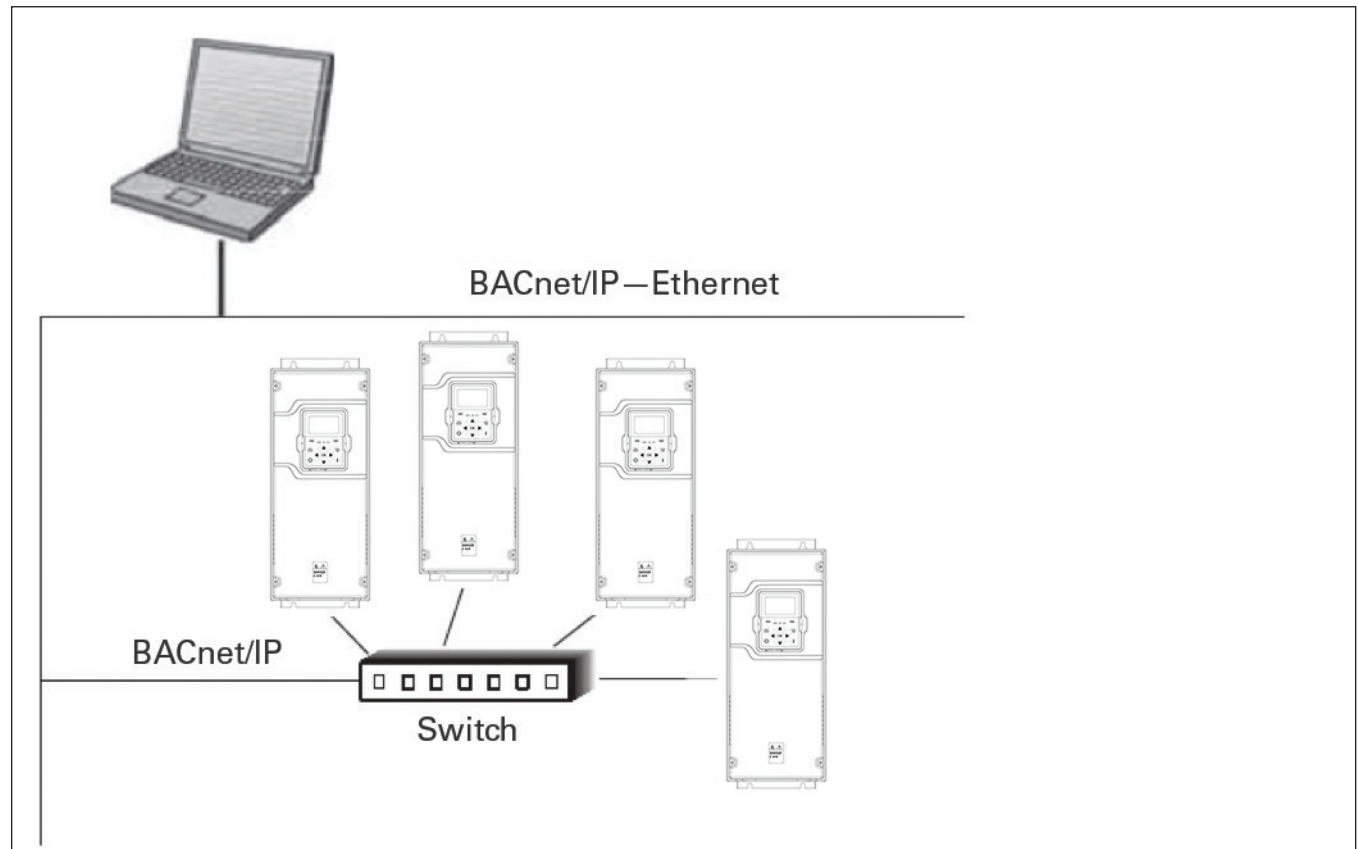
Figure 39. Principle example diagram of BACnet.
