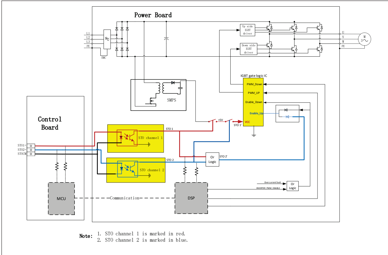
Figure 31. Reliability block diagram.
