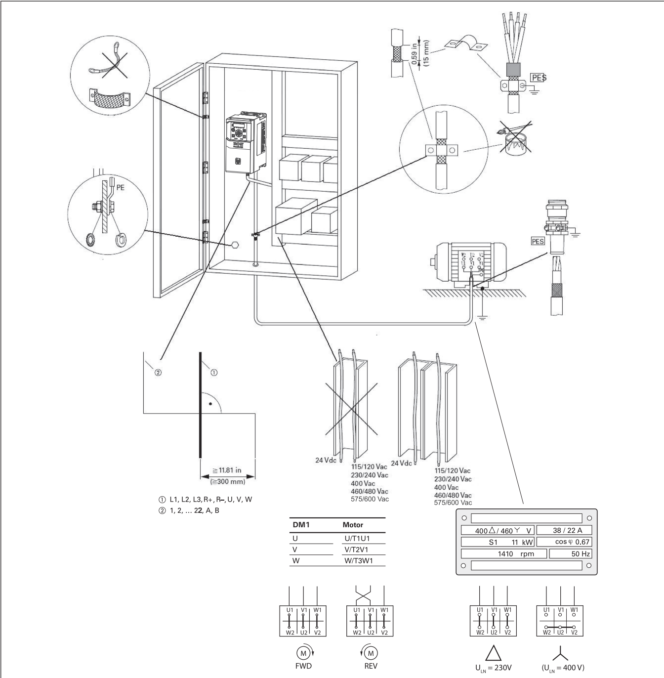
Figure 8. EMC-compliant setup - 230 Vac, 460/480 Vac, 600 Vac.
