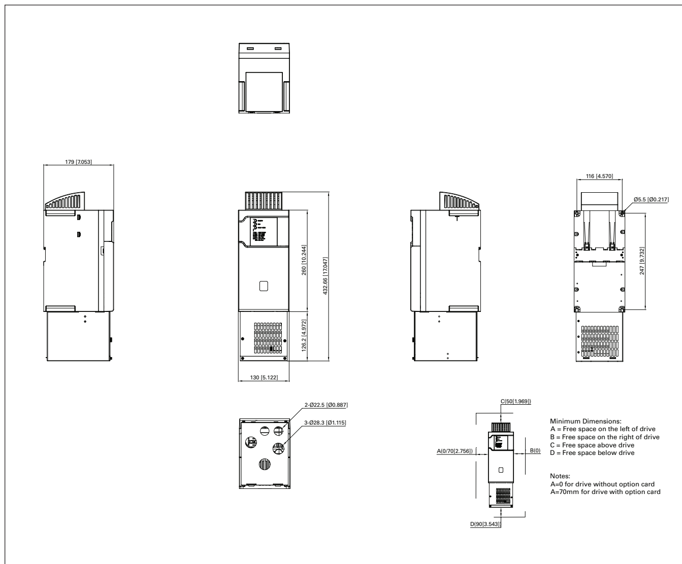
Figure 27. DM1 FR3 with NEMA 1 kit dimension drawing.
