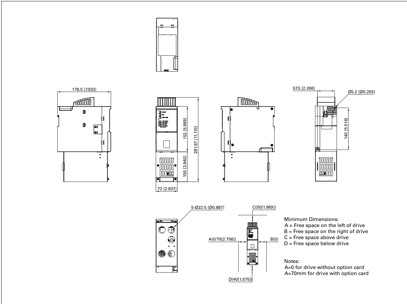
Figure 21. DM1 FR4 without NEMA 1 kit dimension drawing.
