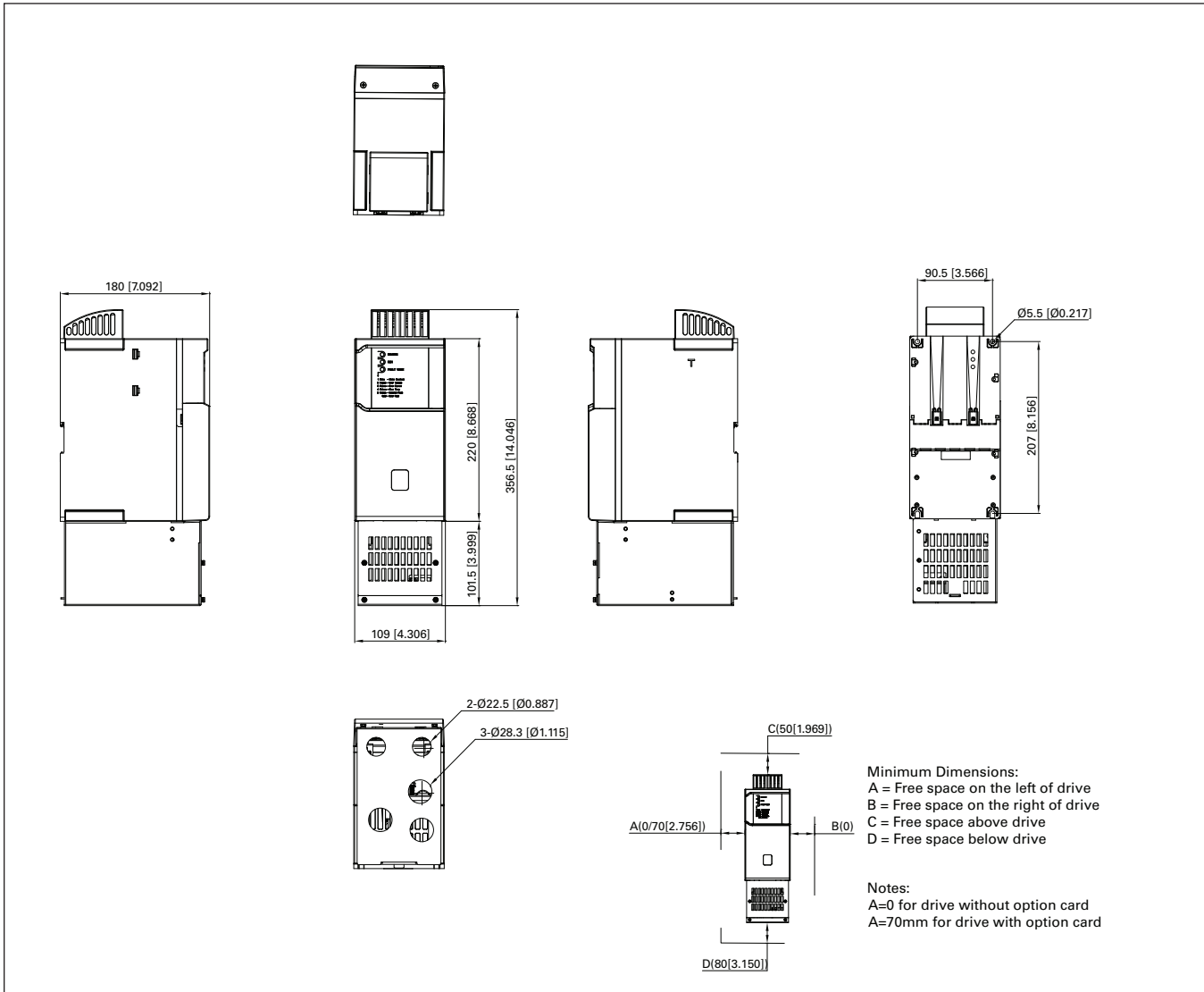
Figure 25. DM1 FR2 with NEMA 1 kit dimension drawing.
