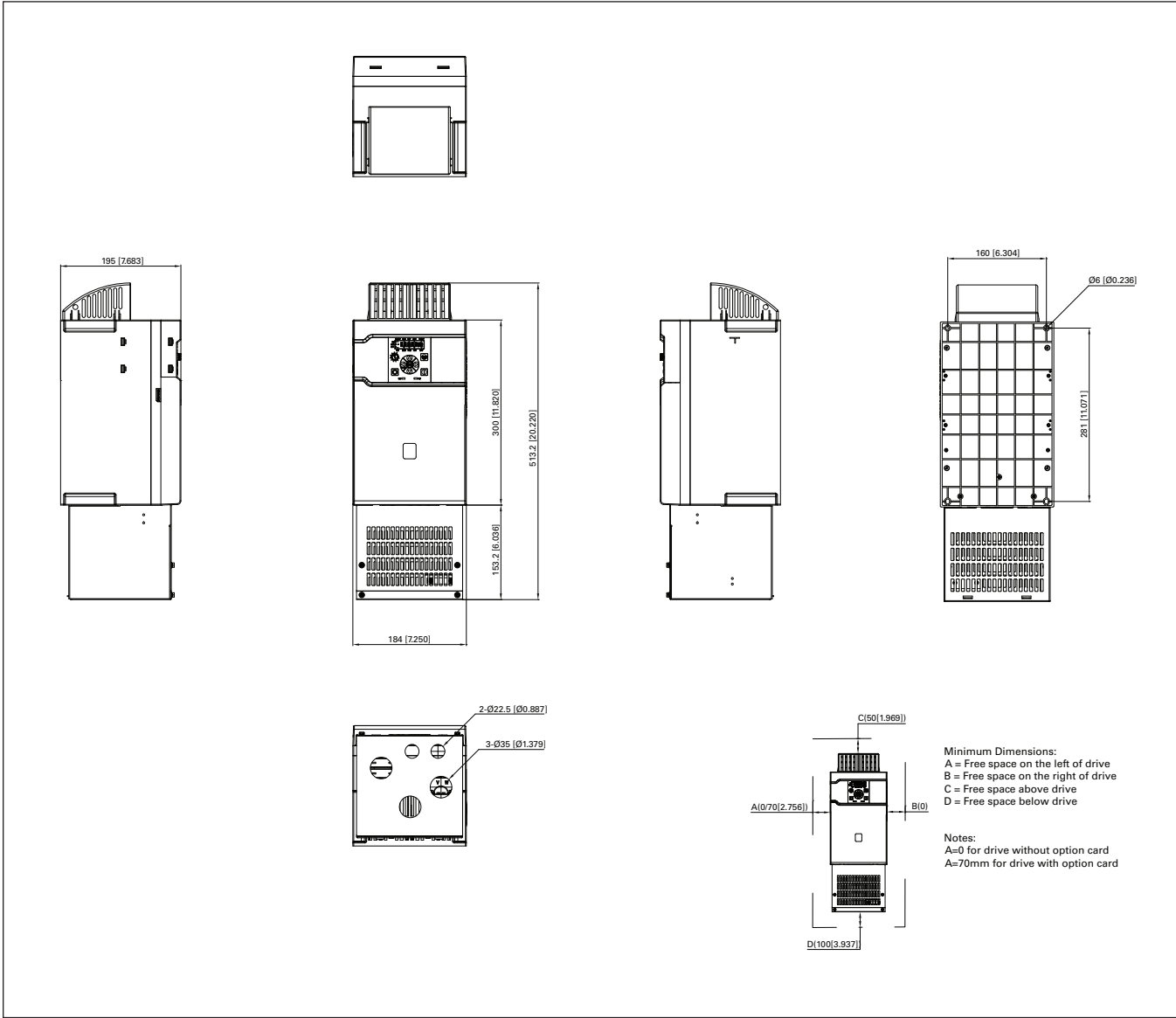
Figure 28. DM1 Pro FR4 with NEMA 1 kit dimension drawing.
