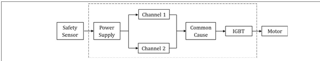
Figure 31. Reliability block diagram.
