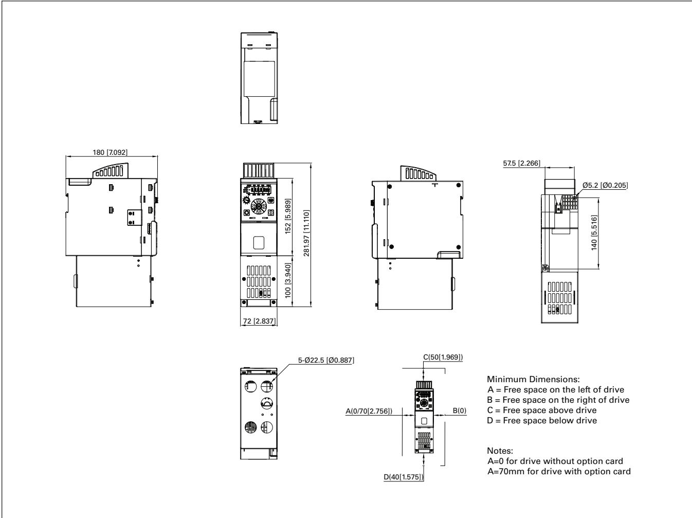
Figure 22. DM1 Pro FR1 with NEMA 1 kit dimension drawing.
