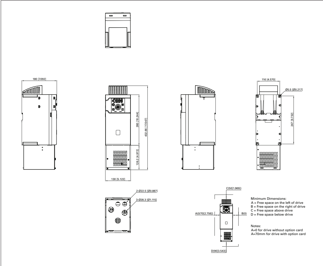
Figure 26. DM1 Pro FR3 with NEMA 1 kit dimension drawing.
