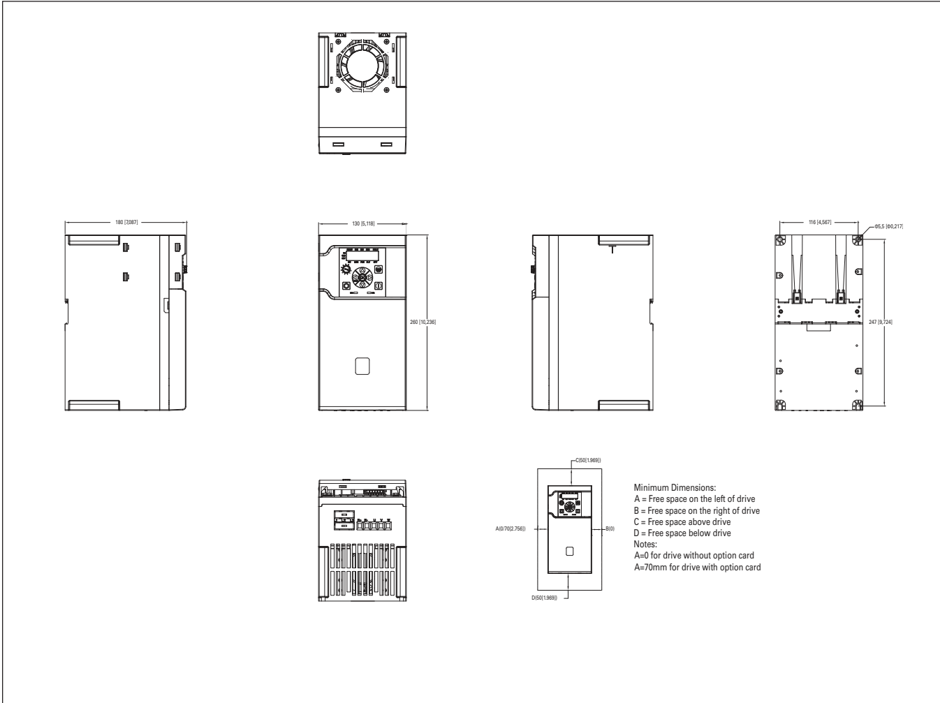
Figure 16. DM1 Pro FR3 without NEMA 1 kit dimension drawing.
