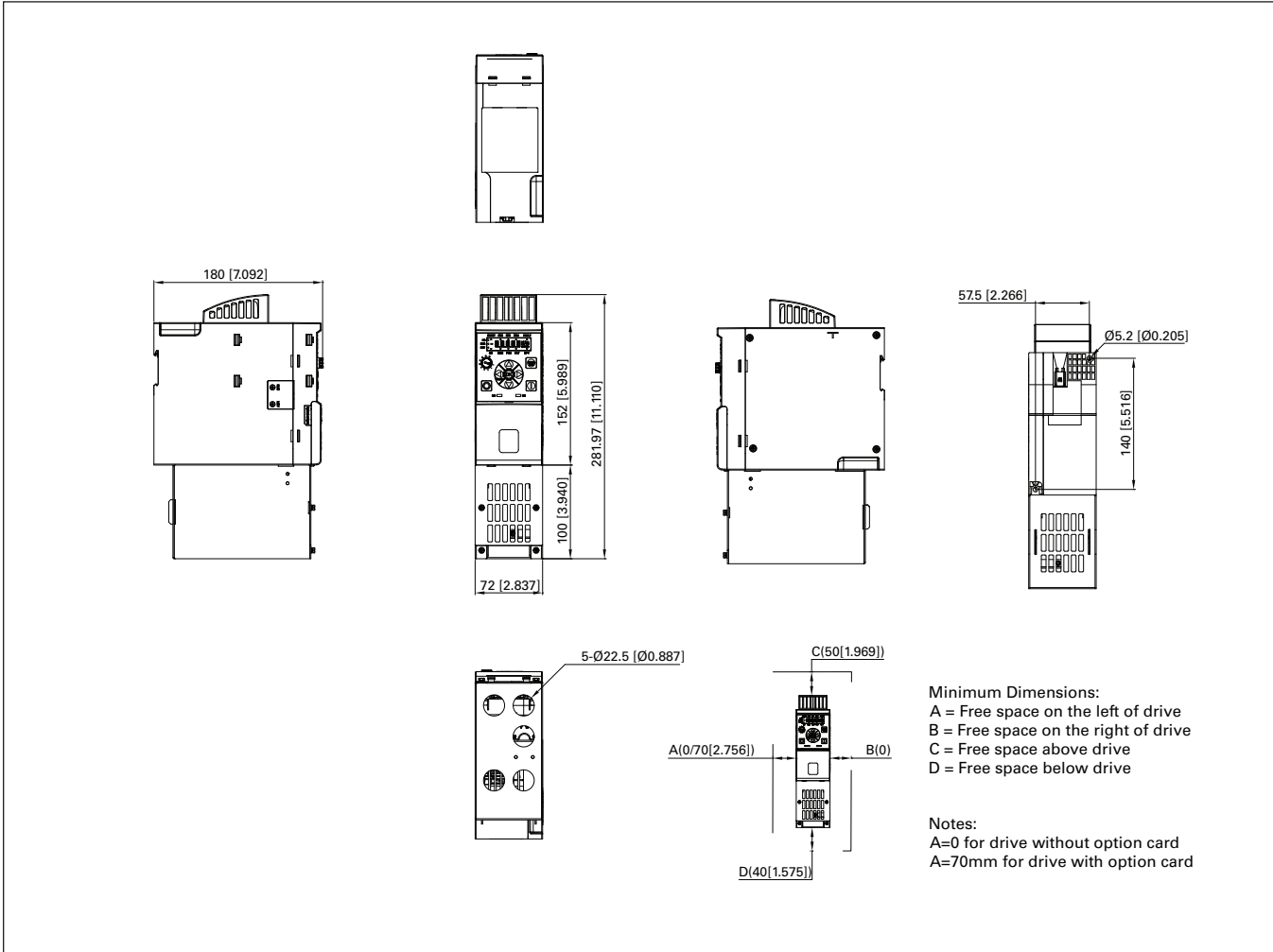
Figure 20. DM1 FR4 without NEMA 1 kit dimension drawing.
