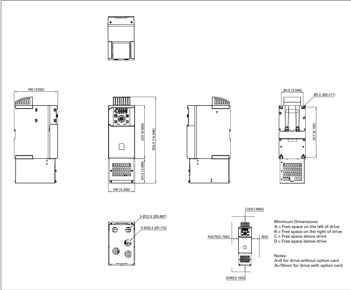
Figure 24. DM1 Pro FR2 with NEMA 1 kit dimension drawing.
