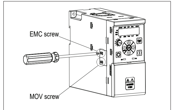
Figure 11. Location of the EMC/MOV screws in frame 2-4.
