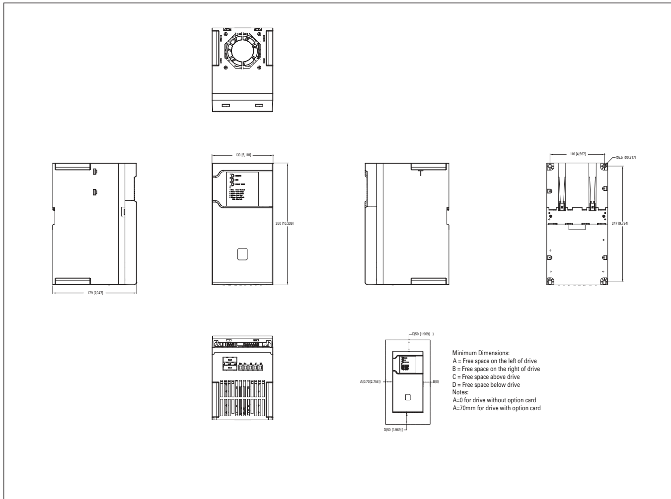
Figure 17. DM1 FR3 without NEMA 1 kit dimension drawing.
