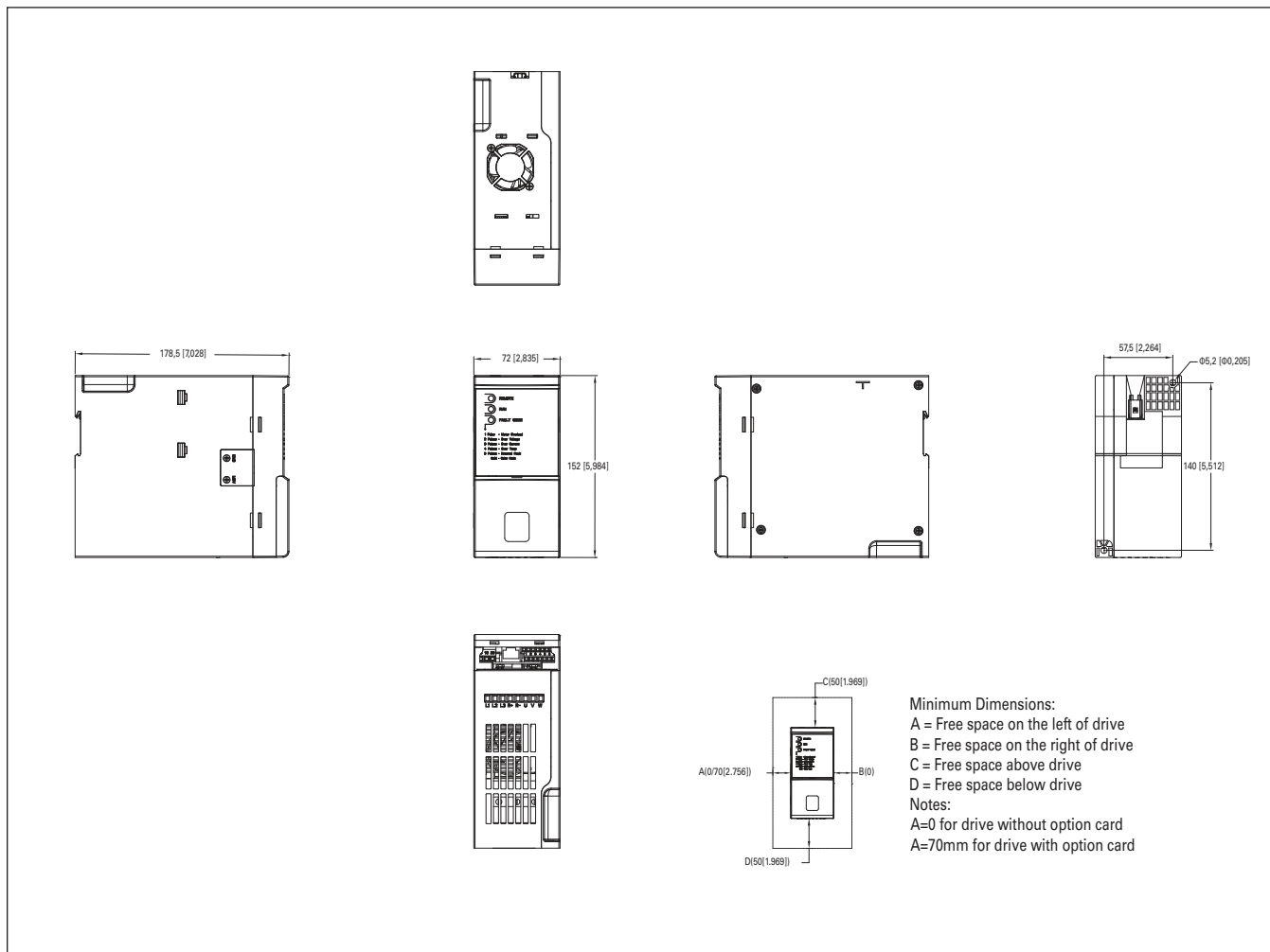
Figure 13. DM1 FR1 without NEMA 1 kit dimension drawing.
