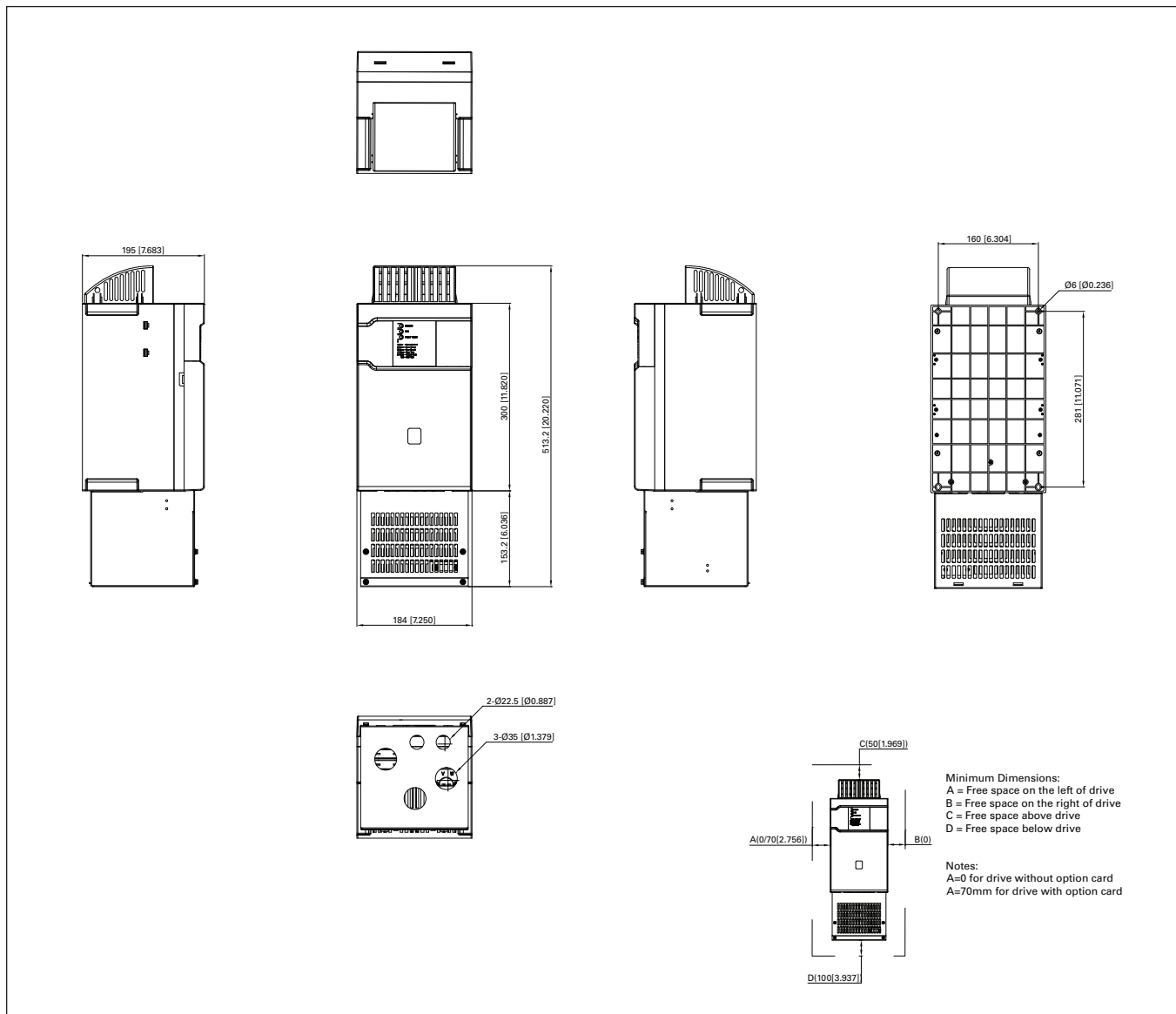
Figure 29. DM1 FR4 with NEMA 1 kit dimension drawing.
