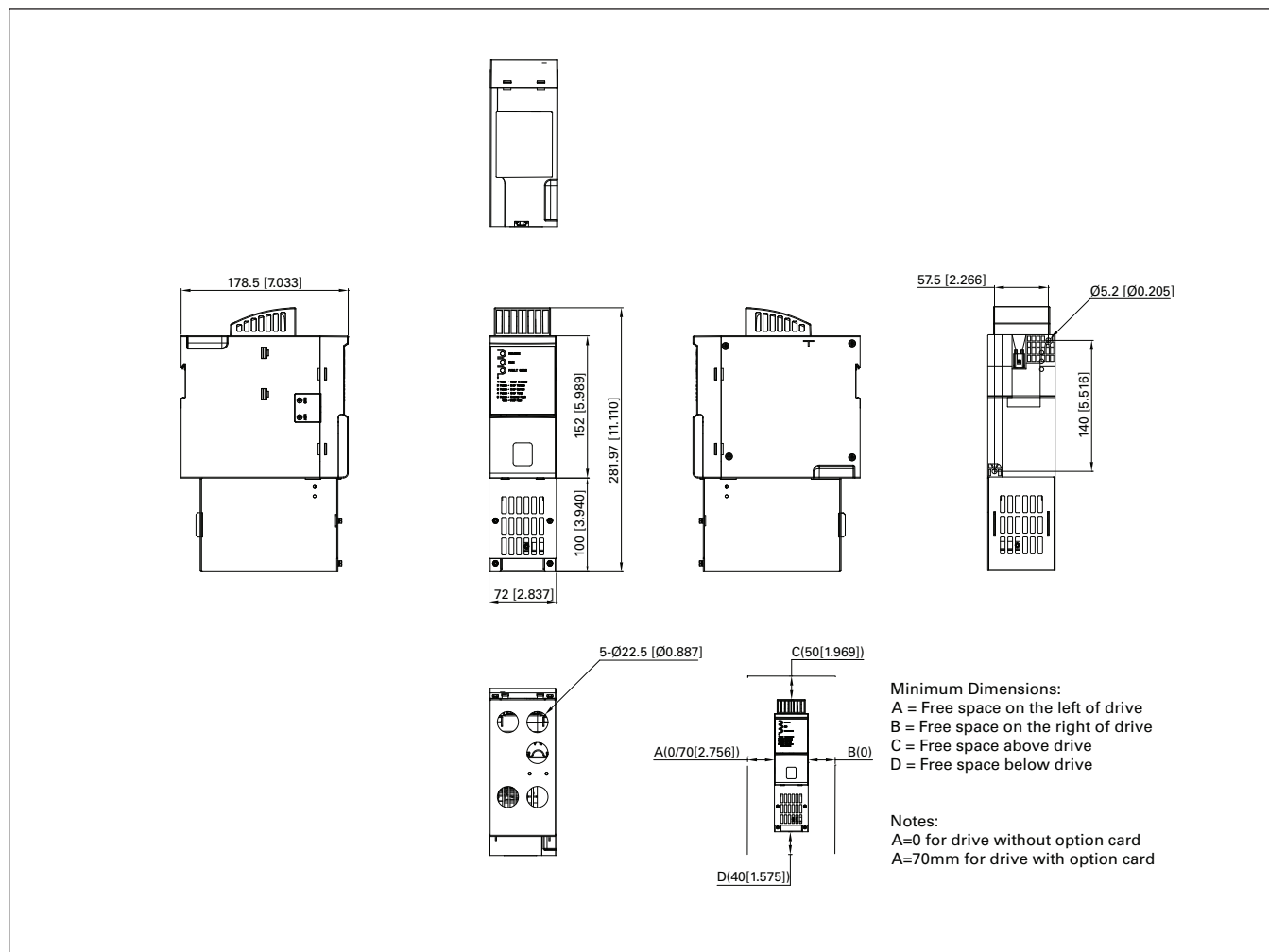
Figure 23. DM1 FR1 with NEMA 1 kit dimension drawing.
